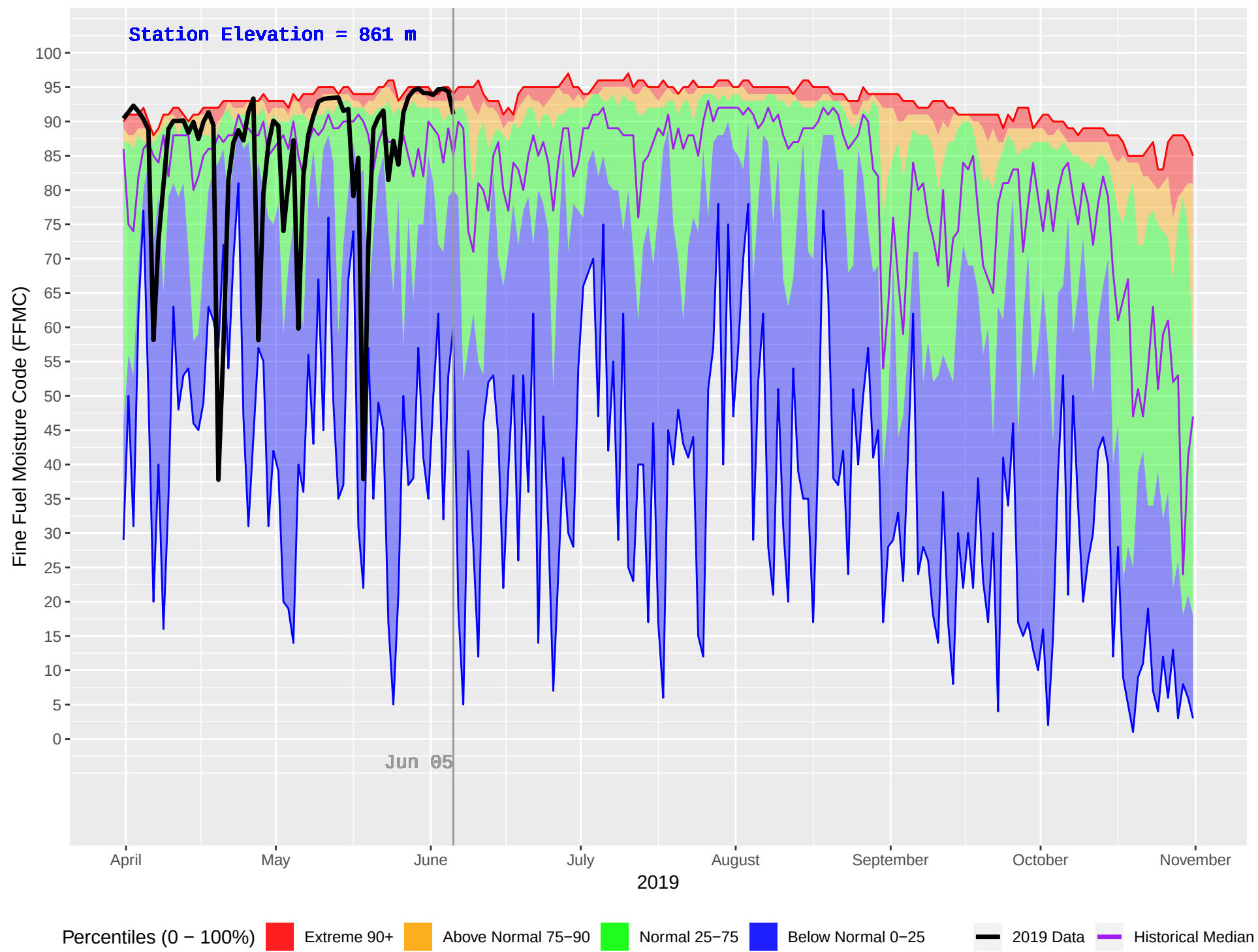
BLAEBERRY (866) : Historical (2004–2018) and Current (2019) Daily Fine Fuel Moisture Code (FFMC)
