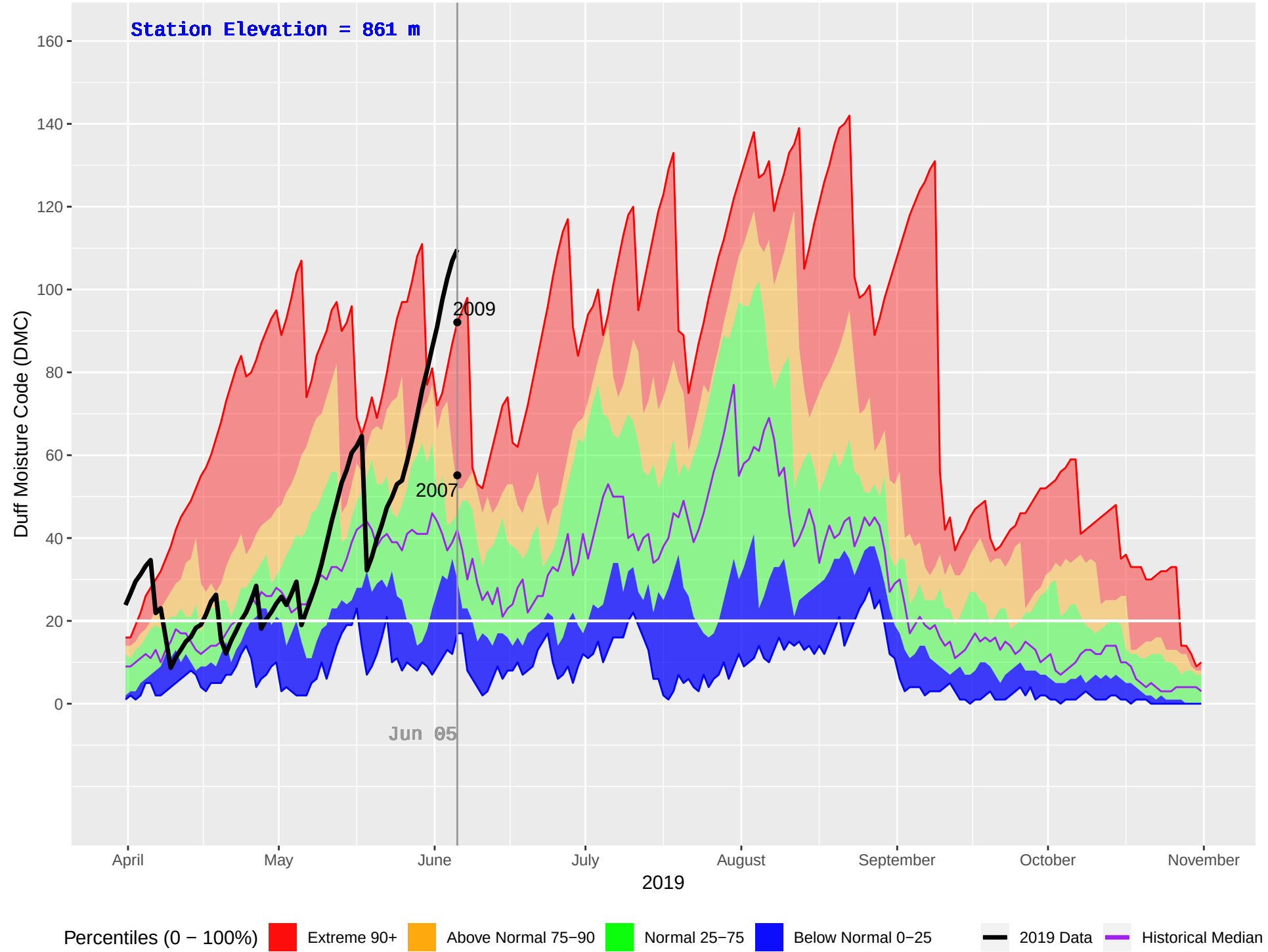
BLAEBERRY (866) : Historical (2004–2018), Current (2019) Daily Duff Moisture Code (DMC)
