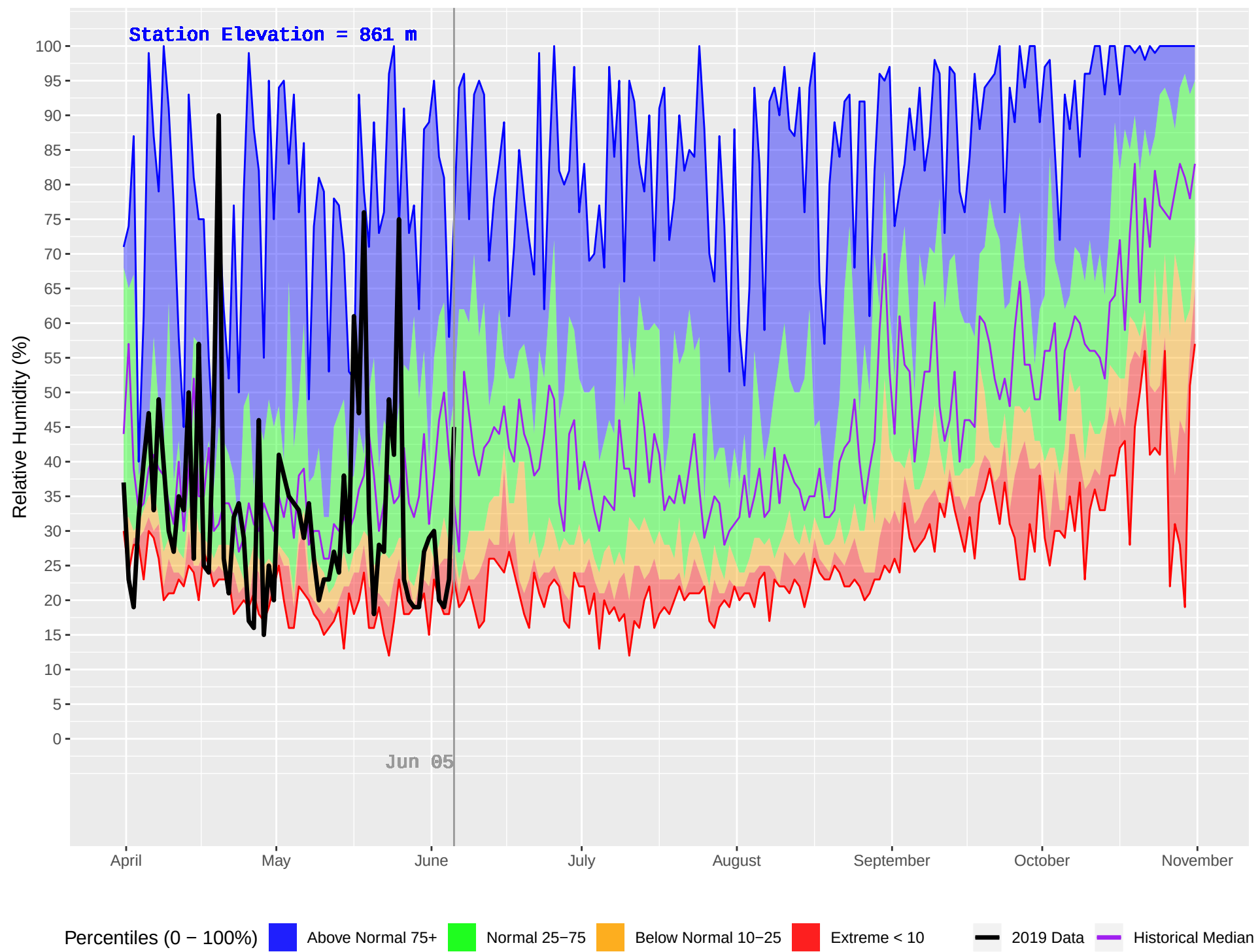
BLAEBERRY (866) : Historical (2004–2018) and Current (2019) Daily Relative Humidity
