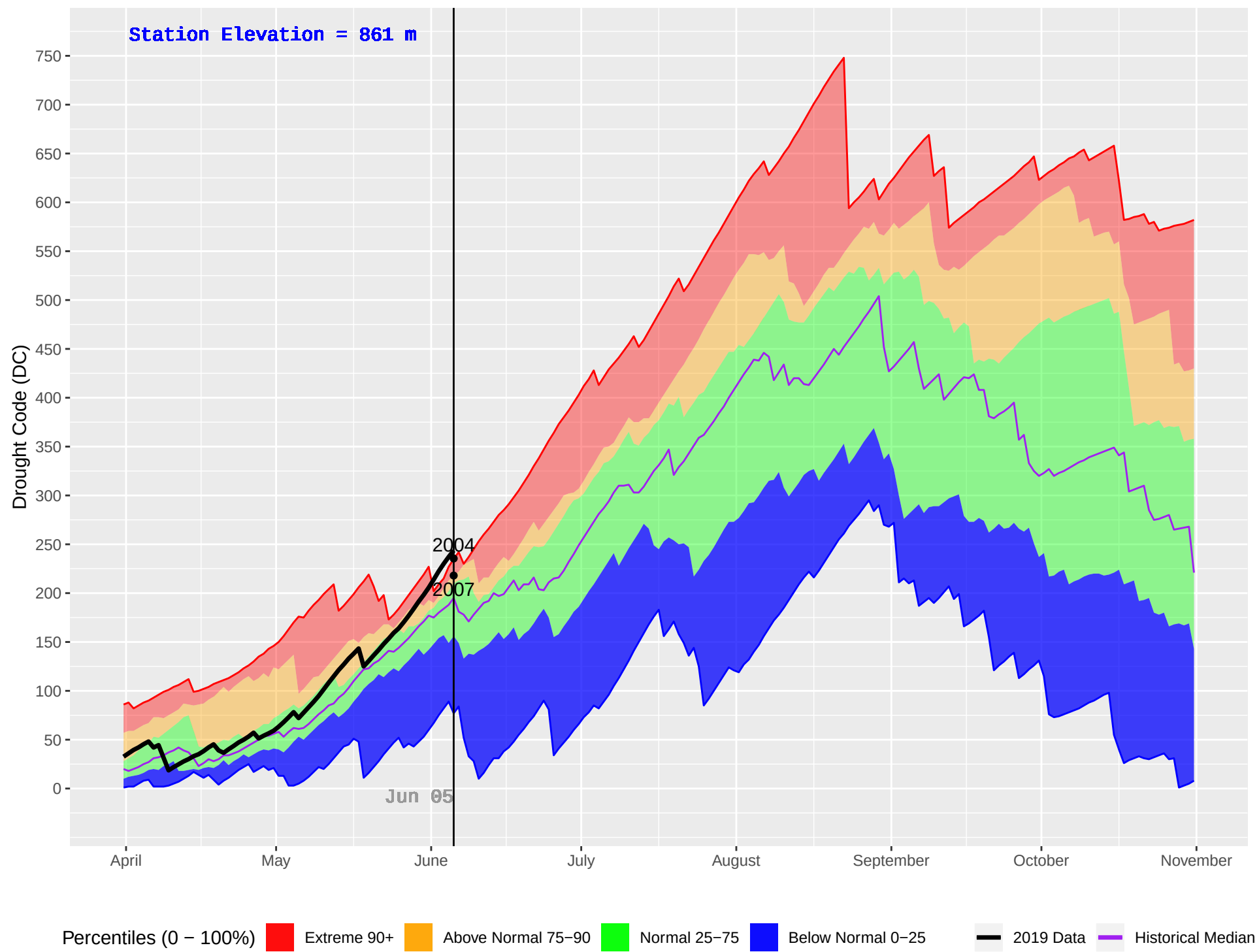
BLAEBERRY (866) : Historical (2004–2018) and Current (2019) Daily Drought Code (DC)
