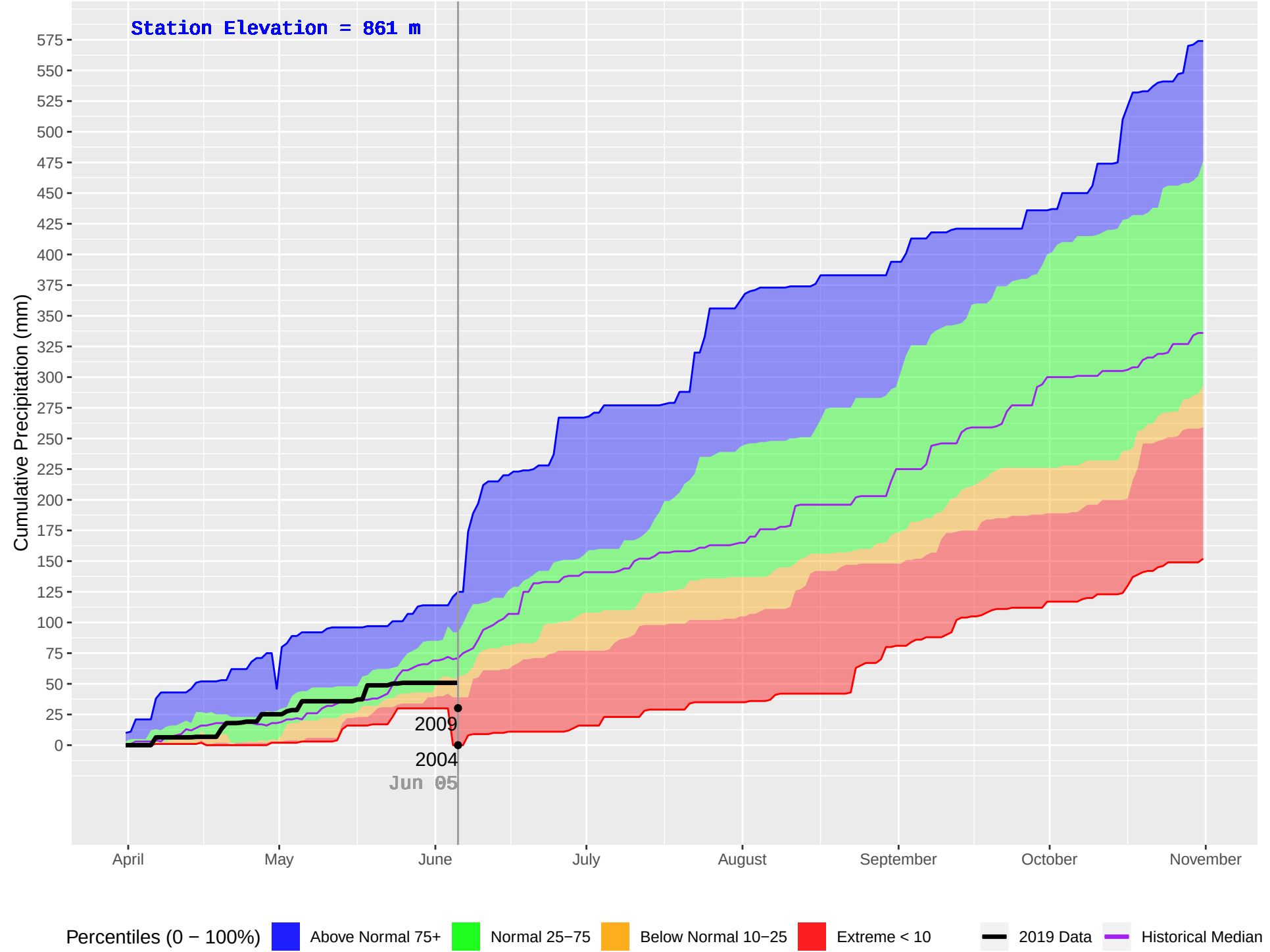
BLAEBERRY (866) : Historical (2004–2018), Current (2019) Daily Cumulative Precipitation
