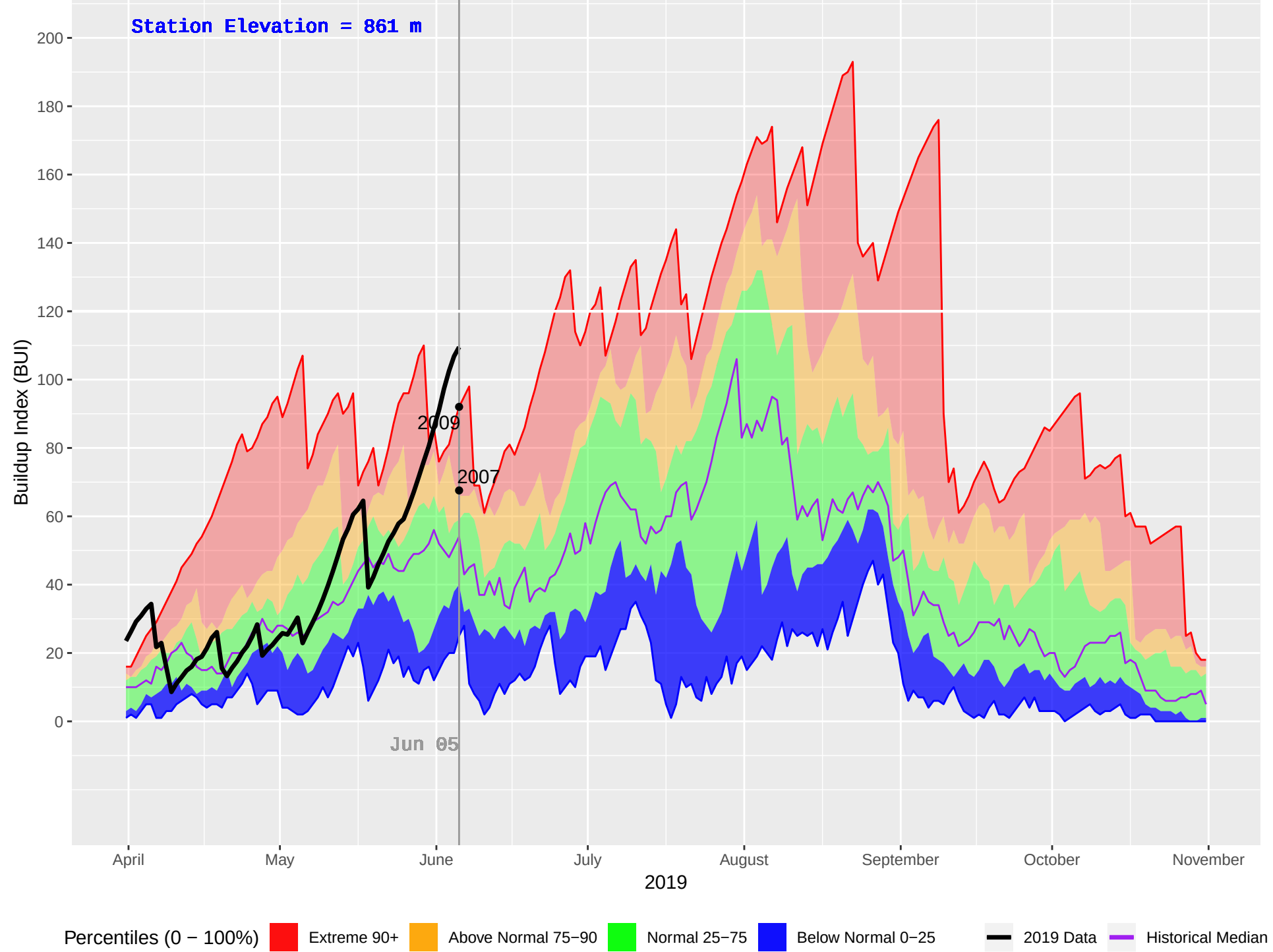
BLAEBERRY (866) : Historical (2004–2018), Current (2019) Daily Buildup Index (BUI)
