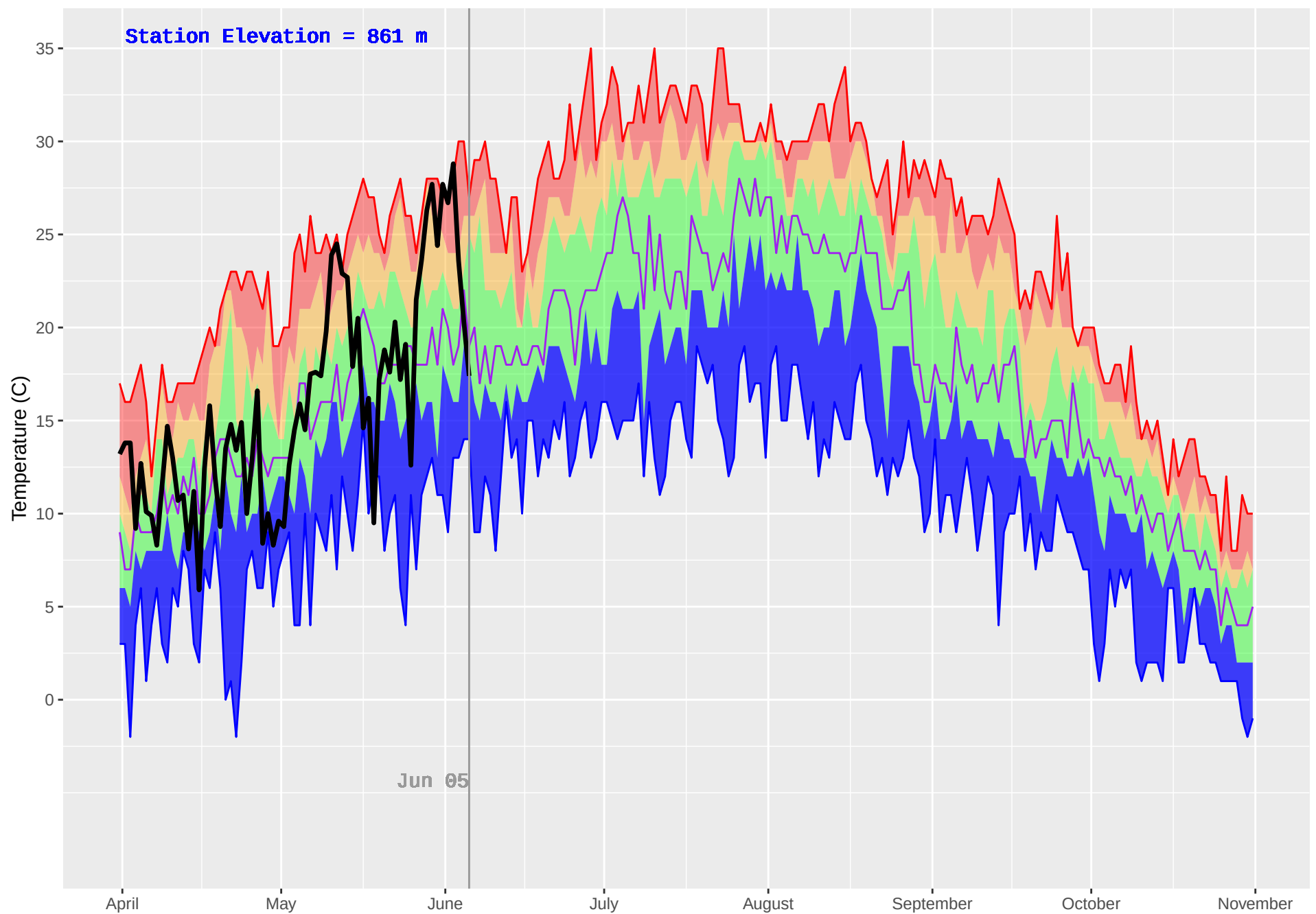
BLAEBERRY (866) : Historical (2004–2018) and Current (2019) Daily Temperature
